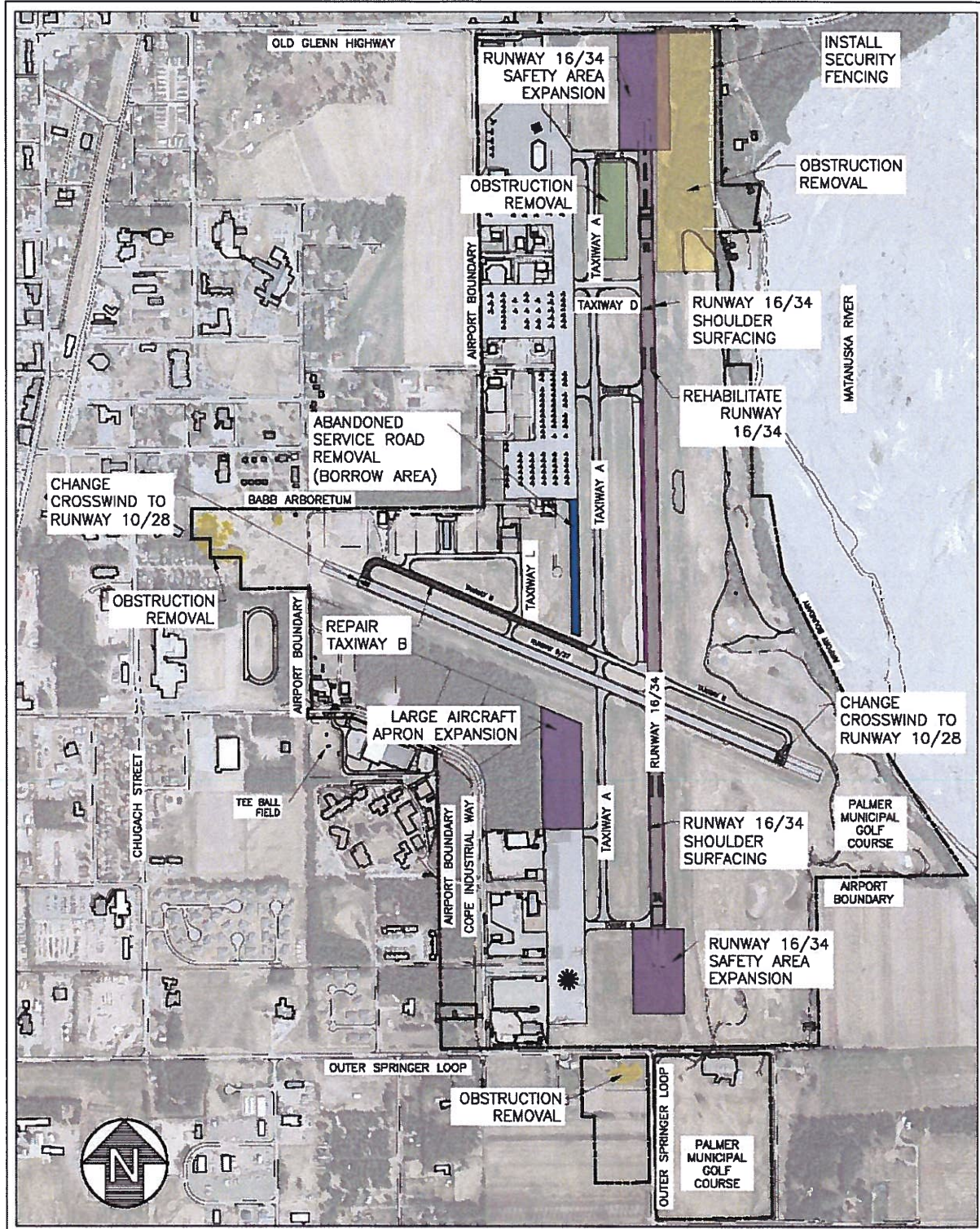
Figure: Rehabilitate Runway 16/34 & Related Improvements
